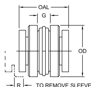
B Type Coupling
