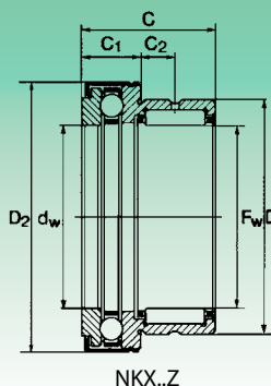
NKX..Z
