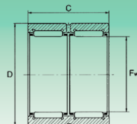
RNA 69..ZW
