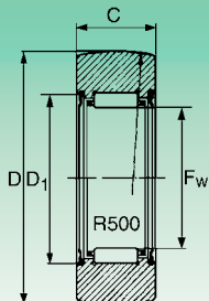
RNA 22..2RS
